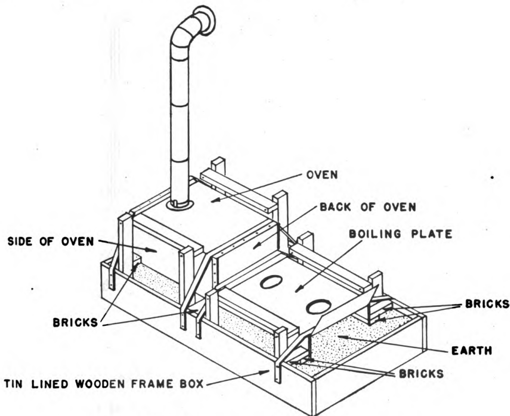
FIGURE 39.—Field range No. 1 installed in baggage car.
