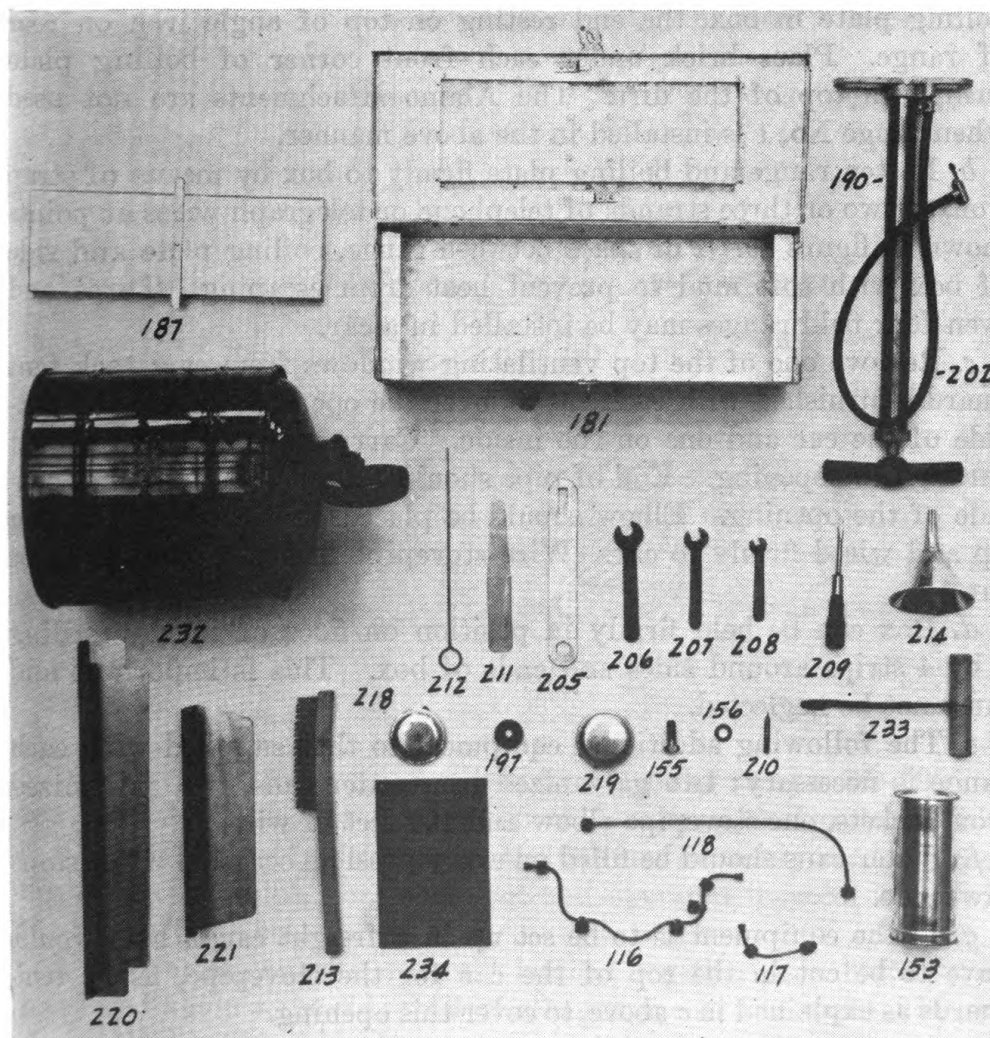
FIGURE 38.—Gasoline fire unit parts and tools—Continued.
