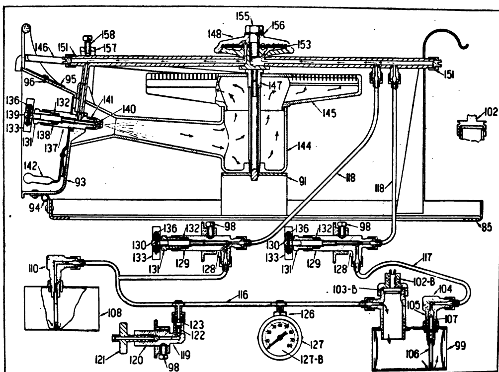
FIGURE 36.—Sectional view of gasoline fire unit.
