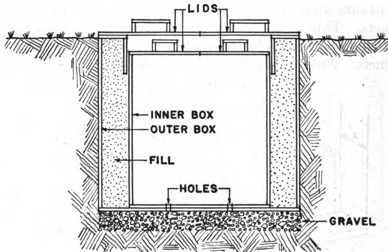
FIGURE 43.—Pit for slops.
