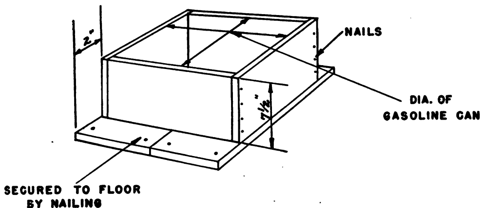
FIGURE 41.—Container for gasoline can.
