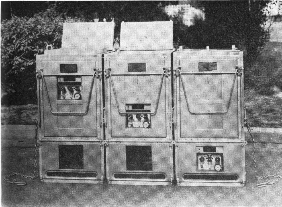
FIGURE 32.—Three units of the range latched together for cooking in transport, showing tie-in chains for anchoring range in truck or railway car. (Right-hand unit is set up for boiling and roasting, middle unit for frying, and left-hand unit for griddle cooking).
