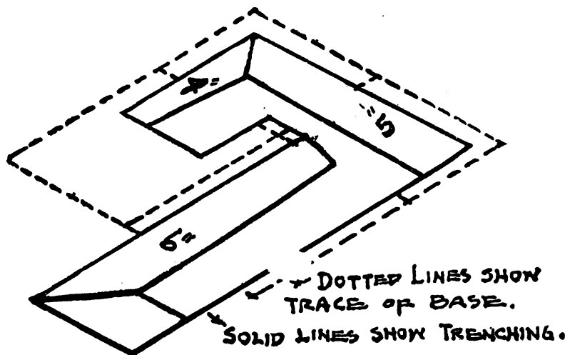
FIGURE 21.—Sketch of trenching for range with attachments.
