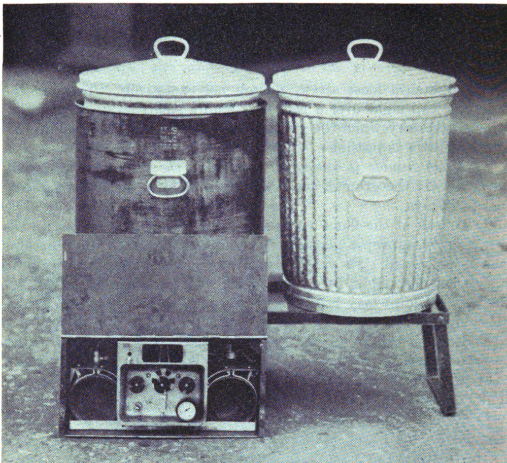
FIGURE 35.—Water heater set up for use, water heater case, water heater can, water heater can cover, and water heater can shield.
