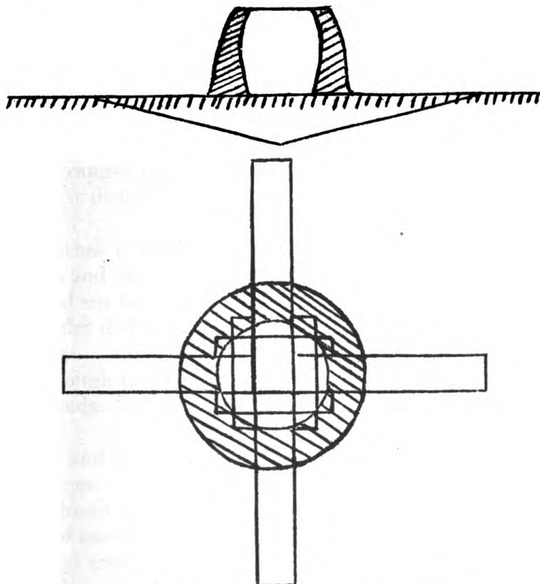
FIGURE 44.—Plan and cross section of company incinerator.
