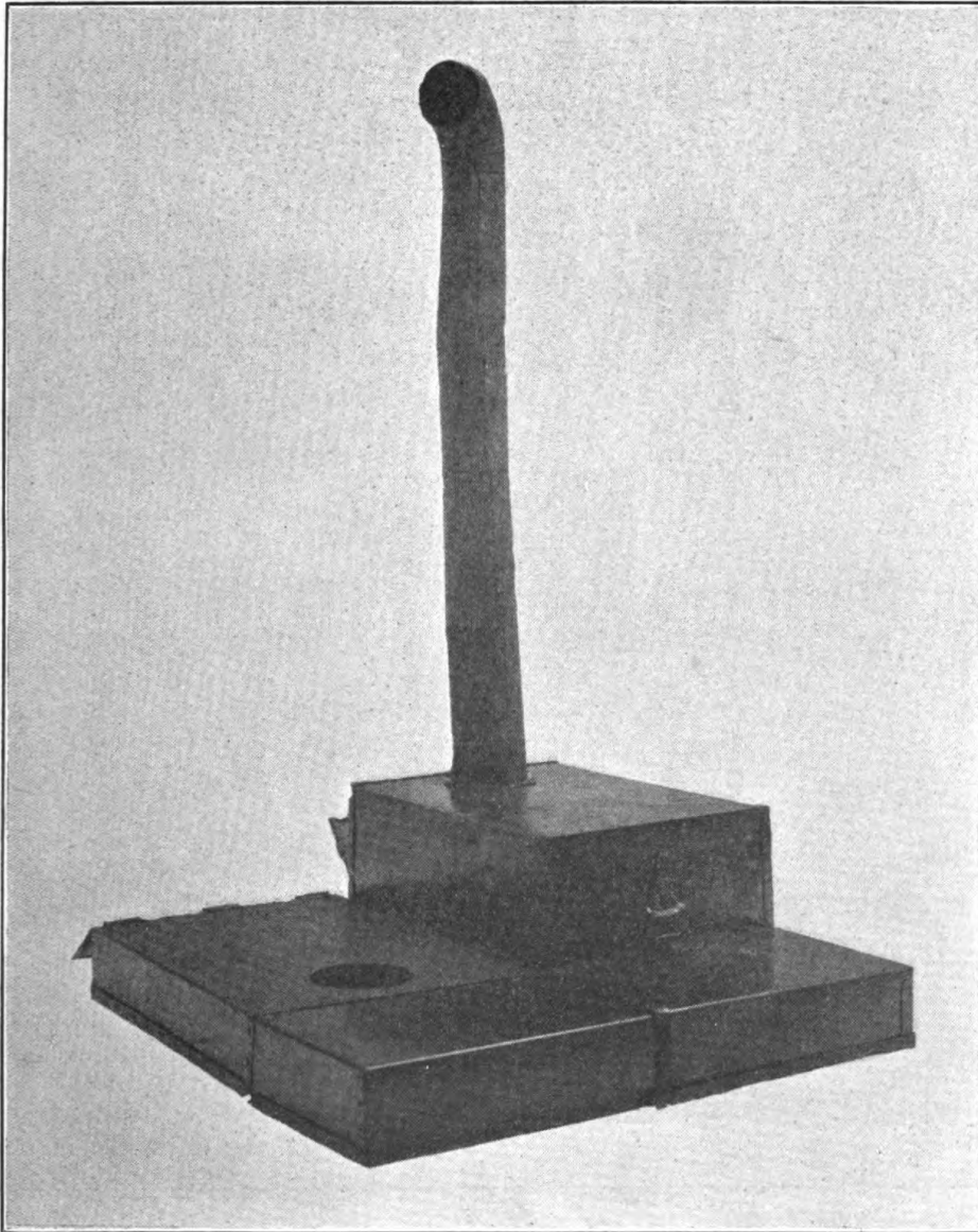
FIGURE 24.—Field range No. 1, set up, rear and right side, with boiling plate and Alamo attachments.
