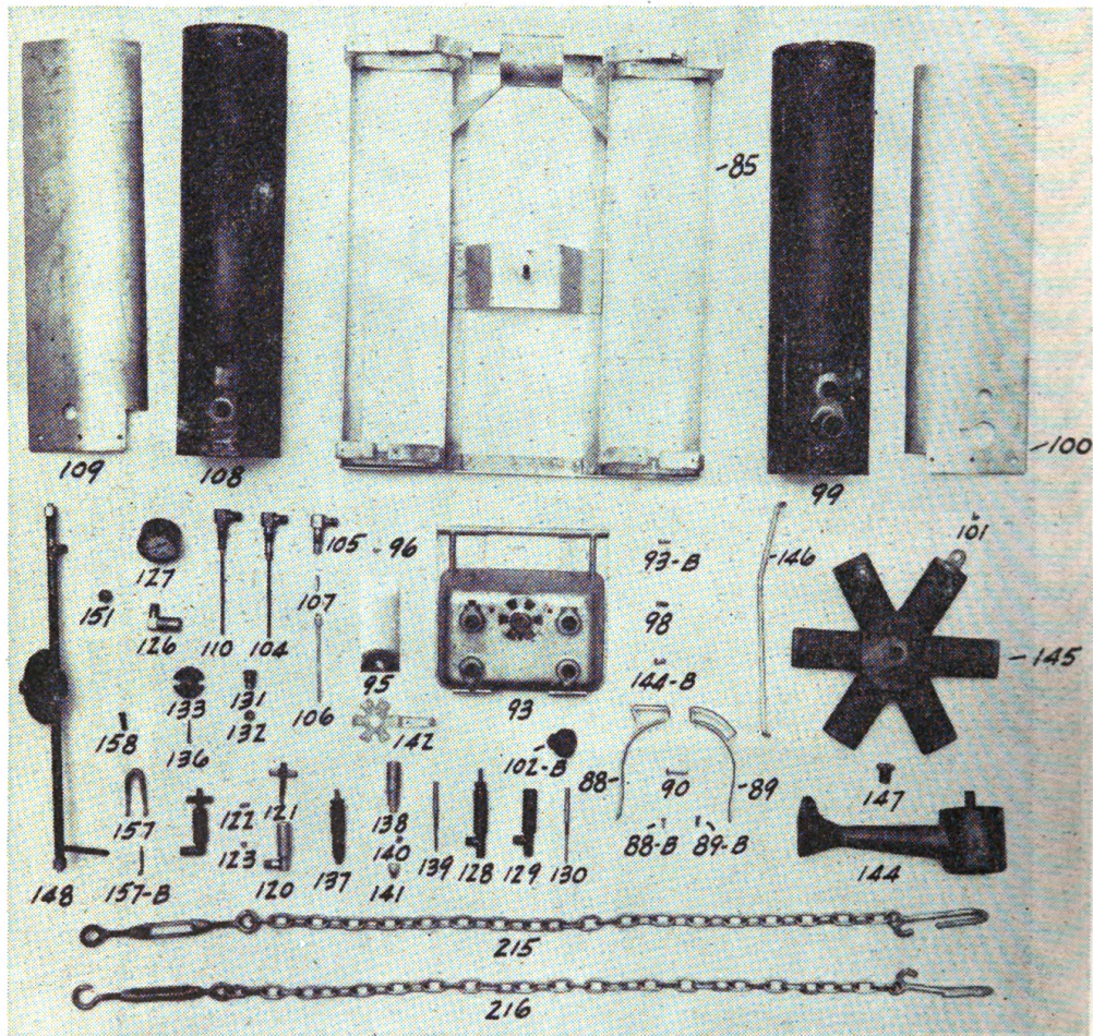
FIGURE 38.—Gasoline fire unit parts and tools.
